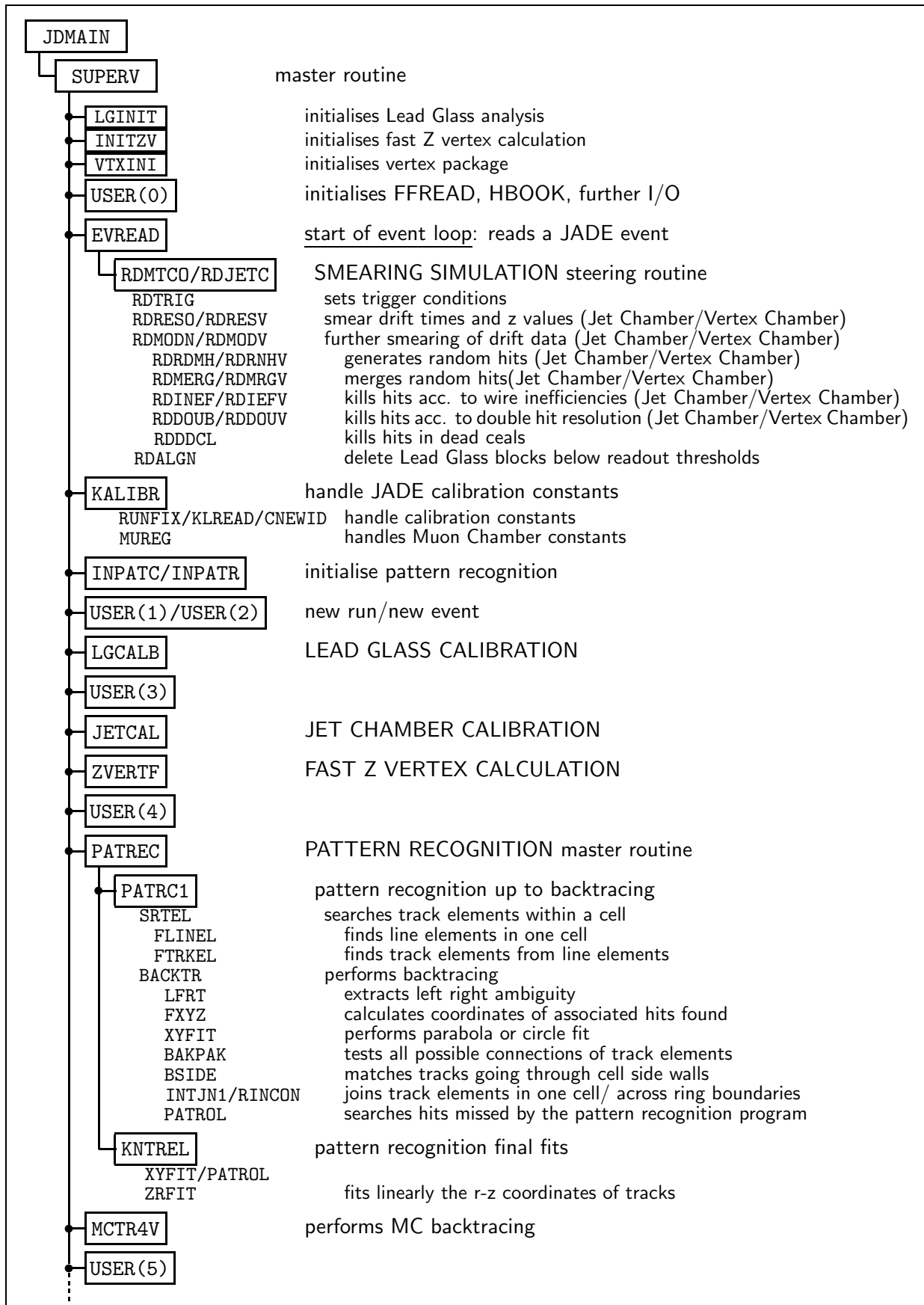
Figure 5: Schematic overview of SUPERV subroutines (part 1).
