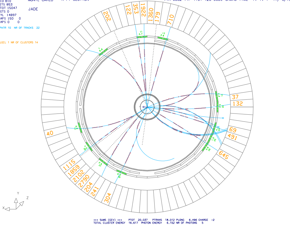
Figure 2: A newly simulated event at \sqrt{s} = 35 GeV displayed by the JADE interactive graphics program JADEZ in the r - \phi projection. The upper plot shows the simulated hits in the Jet Chamber and the Vertex Chamber (including left-right ambiguities), TOF entries and the sum of energies deposited in the Lead Glass. The lower plot represents various results of the event reconstruction. The solid lines represent the tracks found by the pattern recognition programs, the dashed lines indicate the results of the cluster analysis.
