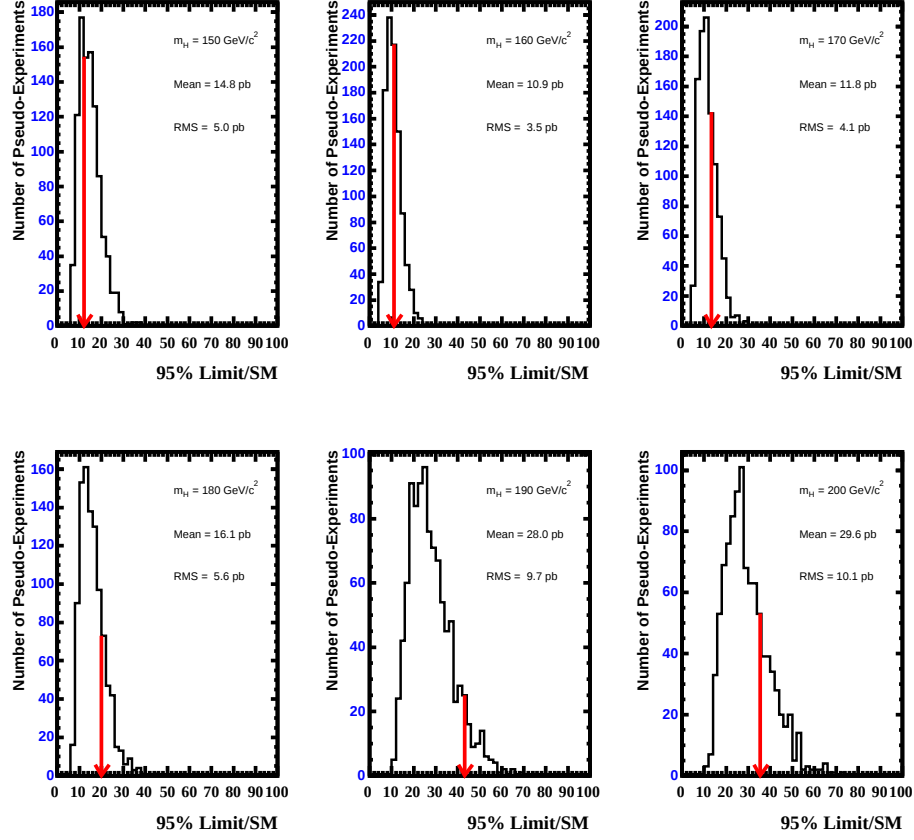
Figure 6: The distributions of upper limits from the pseudo-experiments for Higgs mass between 150 and 200 GeV/c 2 where the arrows indicate the observed 95% upper limit from data.
