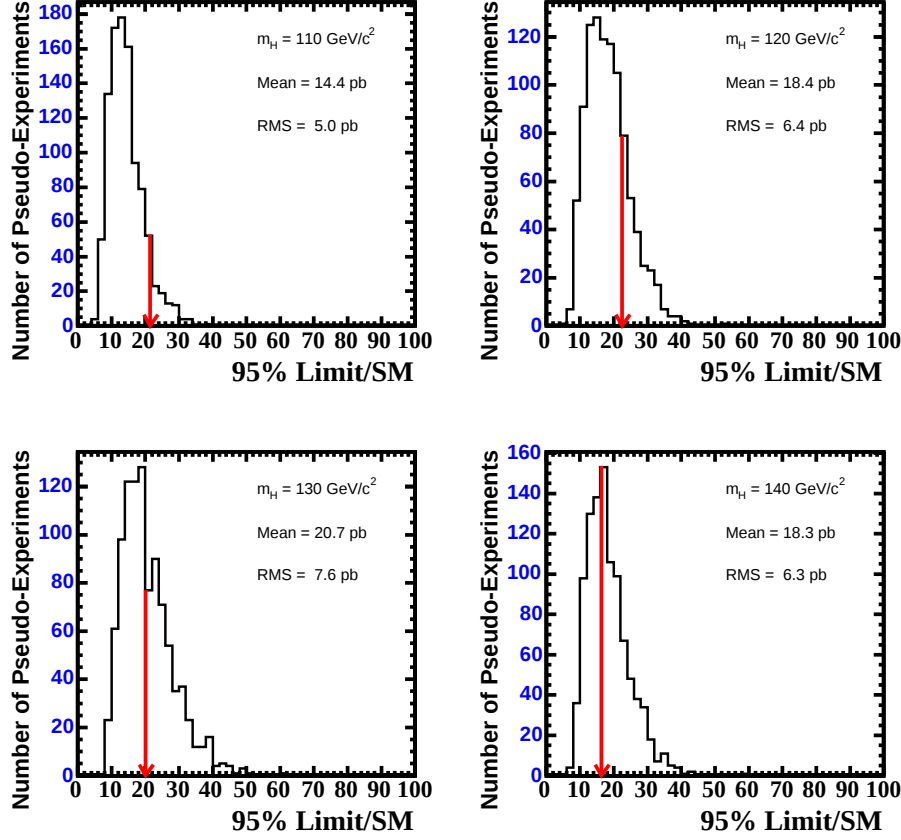
Figure 5: The distributions of upper limits from the pseudo-experiments for Higgs mass between 110 and 140 GeV/c 2 where the arrows indicate the observed 95% upper limit from data.
