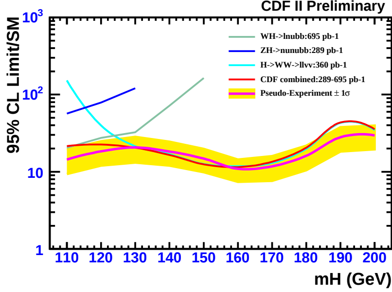
Figure 4: The combined upper limit as function of Higgs masses between 110 and 200 \text{GeV}/c^2 as well as the individual limits from individual channels.
